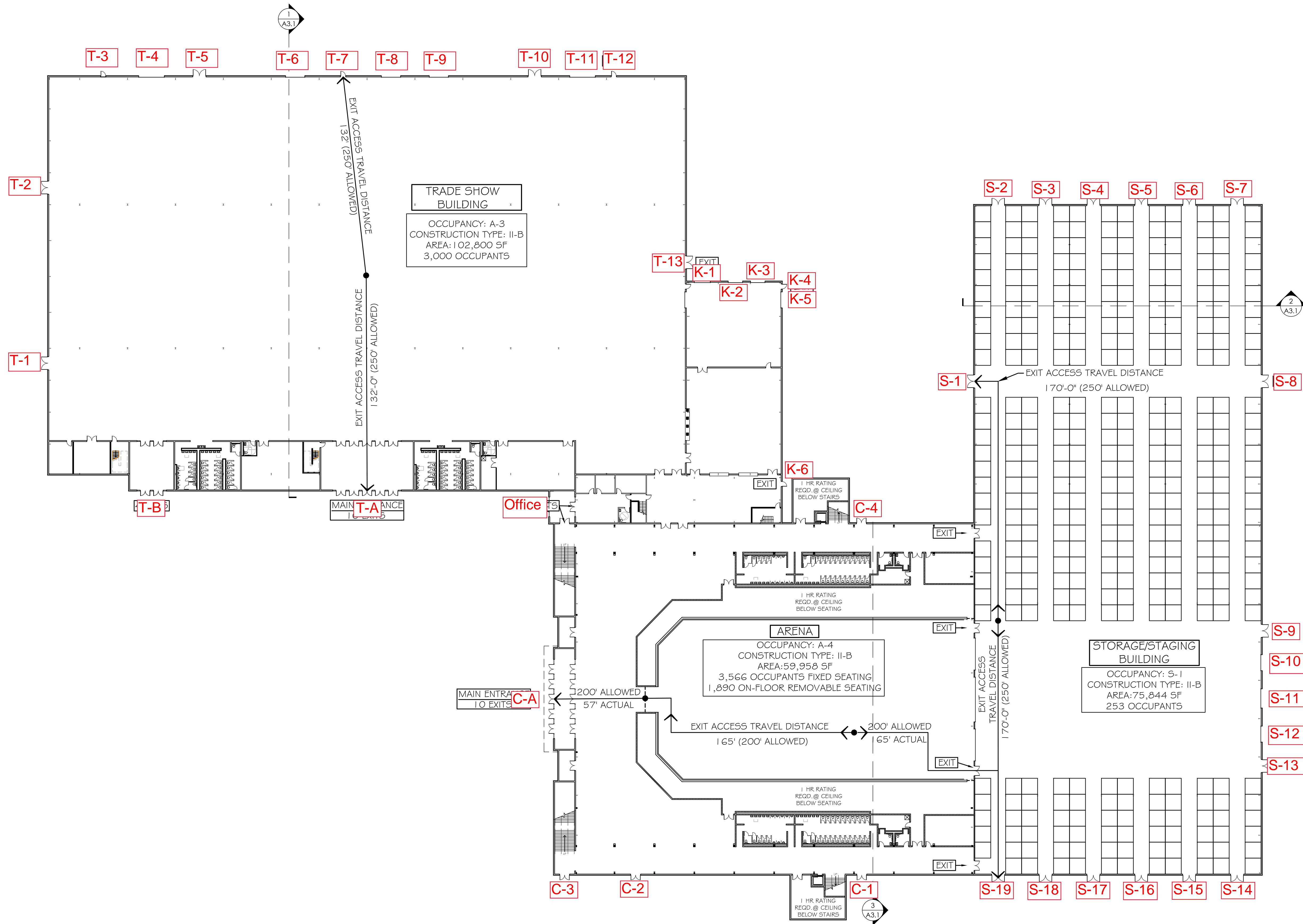
LIFE SAFETY PLAN - MAIN LEVEL SCALE: 1/32" = 1'-0"
